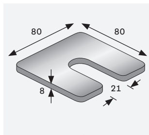
Example: JORDAHL® JVS-80/8-21 horseshoe shim
