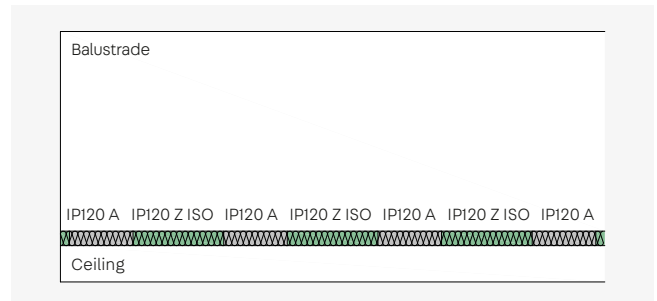
ISOPRO® 120 Z ISO - Use in a parapet
