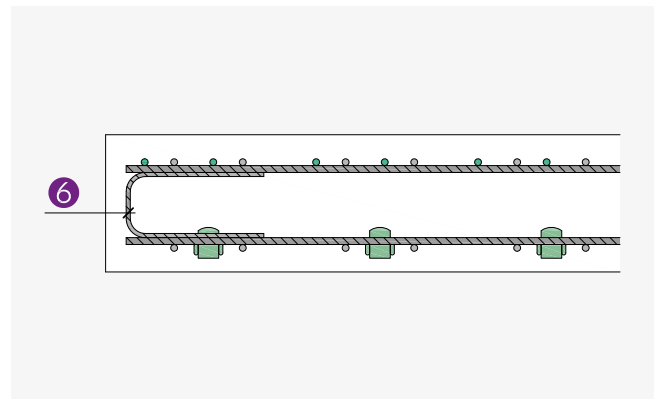
A-A cross-section
