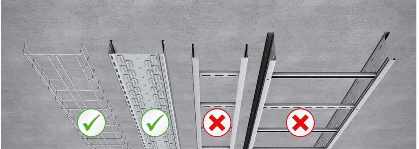
Installation instruction for support systems of wire-mesh cable trays and cable trays attached directly to concrete.
