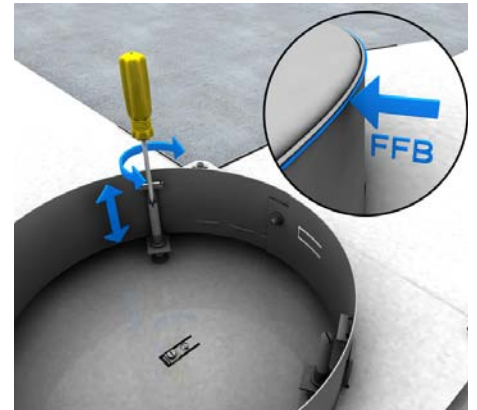
3 | Levelling Adjust the grindable shuttering unit to the height of the finished floor level (FFB) using the levelling screws.
