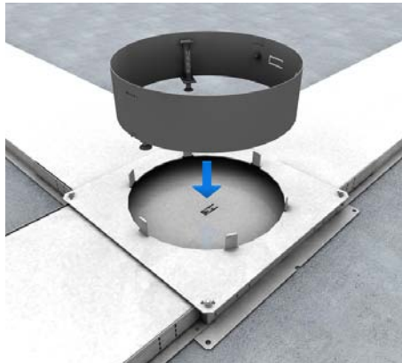
2 | Insert the grindable shuttering unit Insert the grindable shuttering unit into the hollow space floor box from above.
