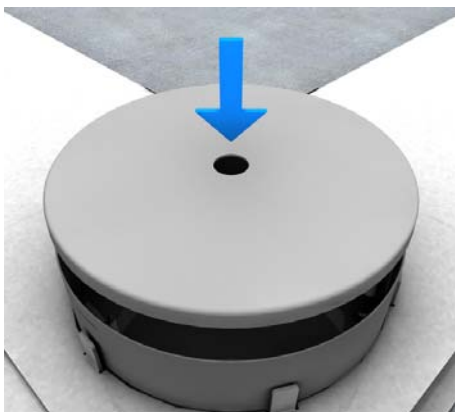
4 | Insert cover Insert the grindable cover in the shuttering unit up to the attachment points. Spray the shuttering unit with form-work oil for an easier removal. Do not use any other separate layers.
