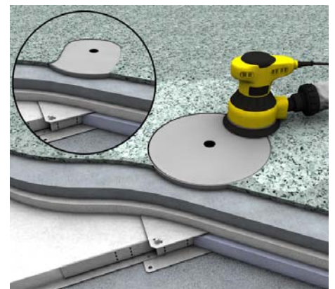
6 | Finished floor level Apply the grindable final layer. Hardening of the new screed layer. Grind multiple times to reach the cover height/final screed height.
