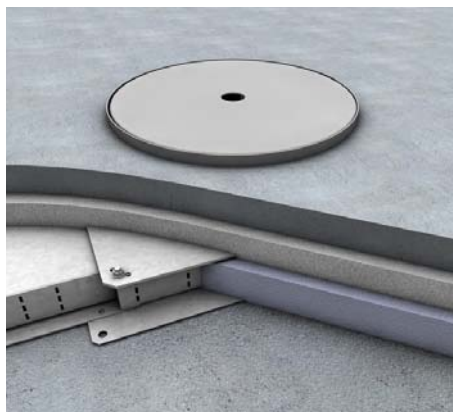
5 | Base screed Insert the insulation, impact noise and base screed layer. Hardening of the screed.
