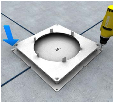
1 | Hollow space floor box Assemble the hollow space floor box on the slab ceiling.
