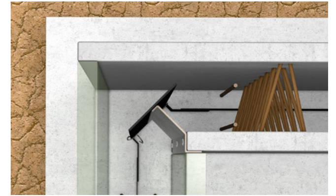
Fig. 2: FTS-Eck for corner joints
