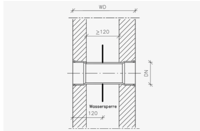
Transwand DM in element wall
