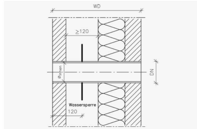
Protective tube in an element wall with interior insulation
