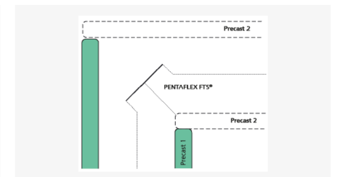
PENTAFLEX® FTS-Eck for corner joints
