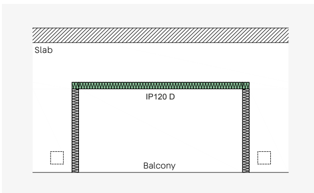
ISOPRO® 120 D - Inset balcony with glass façade, without direct support
