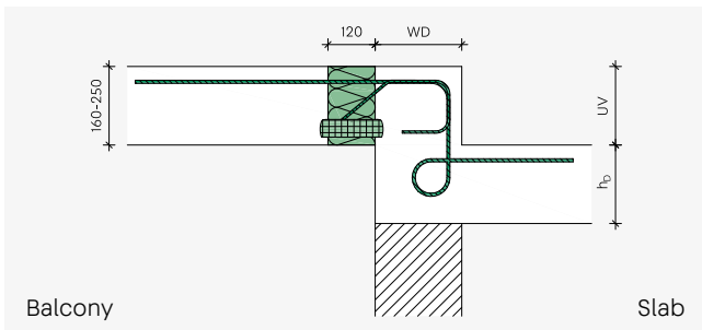
Floors situated at a lower level – ISOPRO® 120 M UV
