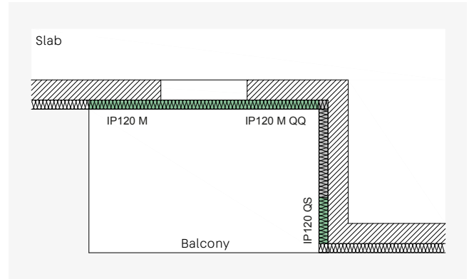
ISOPRO® 120 M - Cantilevered balconies in façade extensions
