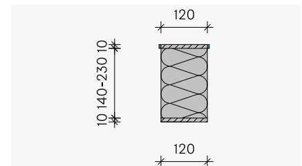
ISOPRO® 120 Z ISO FPI - Cross-section
