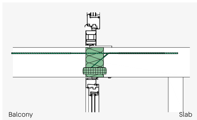
ISOPRO® 120 – installation cross section of glass façade
