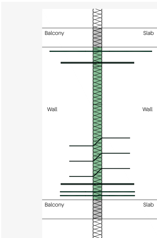
ISOPRO® 120 W - Installation cross-section with wall slab connected to the balcony slab monolithically
