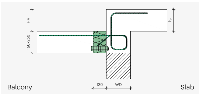
Floors situated at a higher level – ISOPRO® 120 M HV
