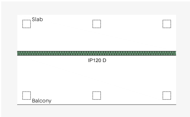
ISOPRO® 120 D - Continuous slab with a glass façade
