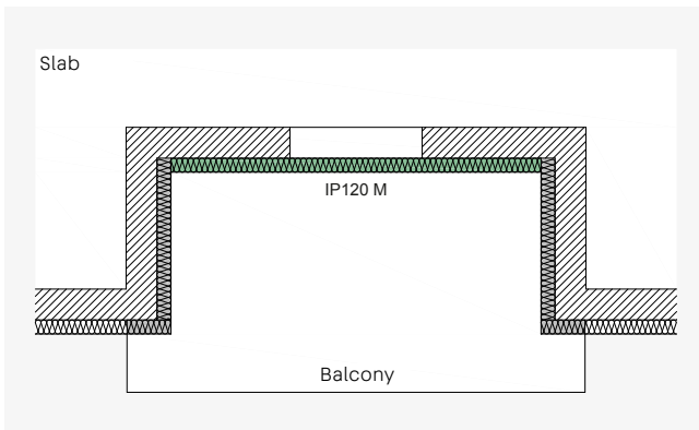
ISOPRO® 120 M - Cantilevered balconies in façade recesses
