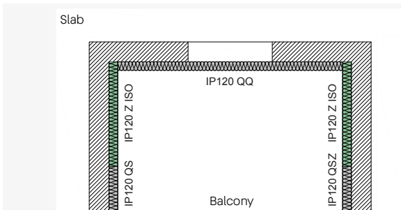
ISOPRO® 120 Z ISO - Loggia with support at specific points
