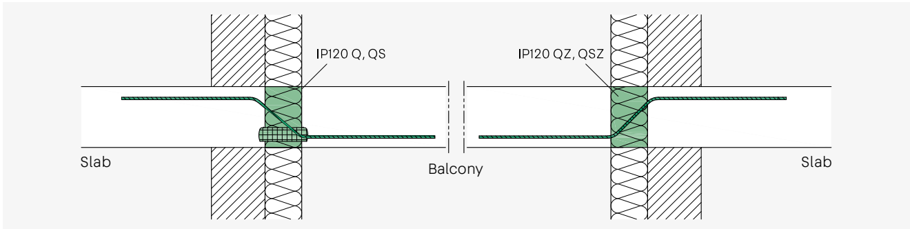
ISOPRO® 120 Q/QZ, QS/QSZ - Installation cross-section with opposite types of the same load class
