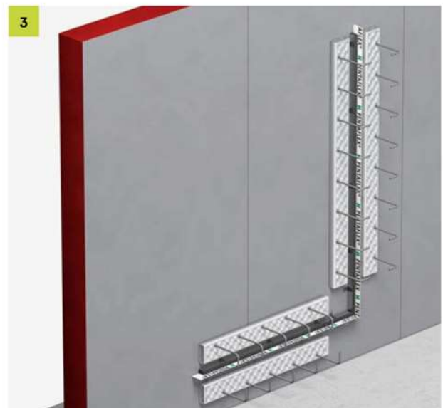
3 Next to the PENTAFLEX® module, nail two single-row FERBOX® backband terminations to the formwork.
