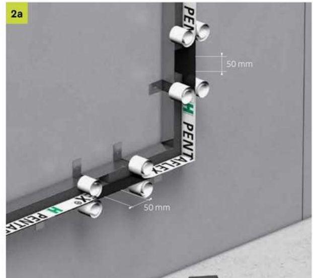
2a Connecting the corner module with two PENTAFLEX® modules Remove the protective film, overlap the sheets by at least 50 mm.
