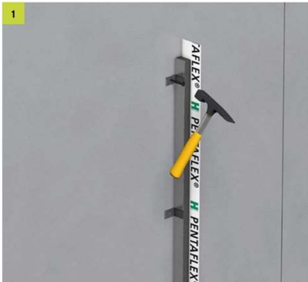
1 Nail the PENTAFLEX® module to the formwork using the nailing lugs.
