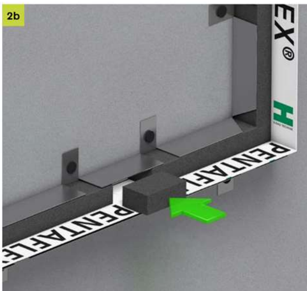
2b Fill empty spaces with EPP plugs
