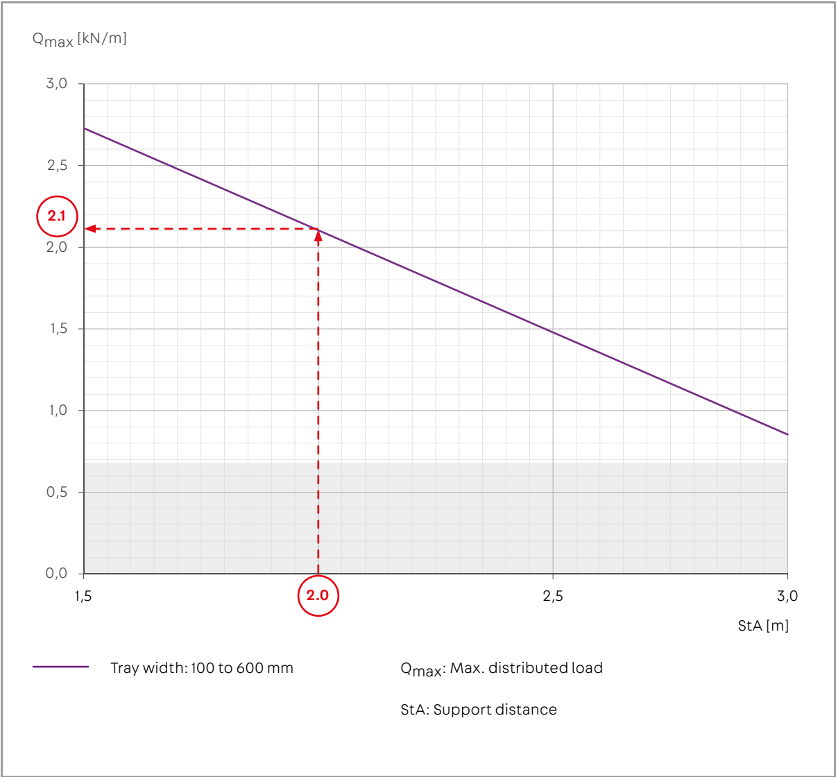
Figure 1: LGG 60 load diagram with the support distance of 2.0 m marked
