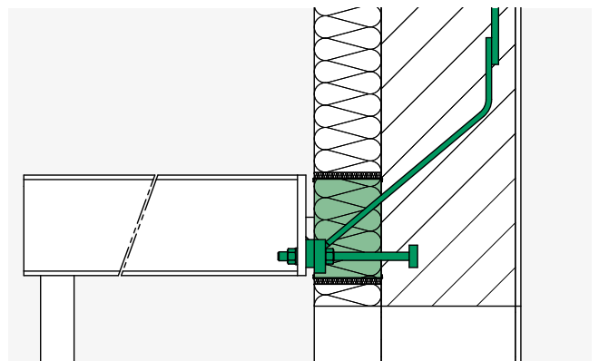
ISOPRO® SQ – Installation cross-section, external thermal insulation composite system, special version for connecting to a wall above:
