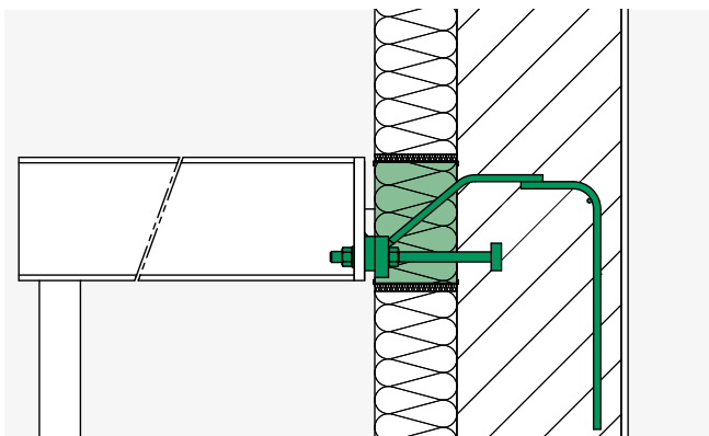
ISOPRO® SQ – Installation cross-section, external thermal insulation composite system, special version for connecting to a wall below:
