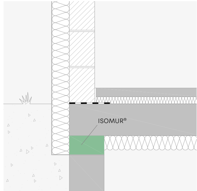
ISOMUR® in the wall below the basement ceiling
