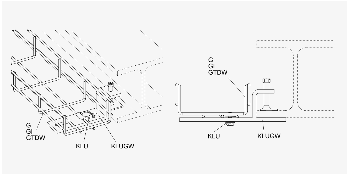
A horizontally aligned U-shaped mesh cable tray mounted on a steel beam using the KLUGW fastening clamp set and the KLU clamp fastening set.
