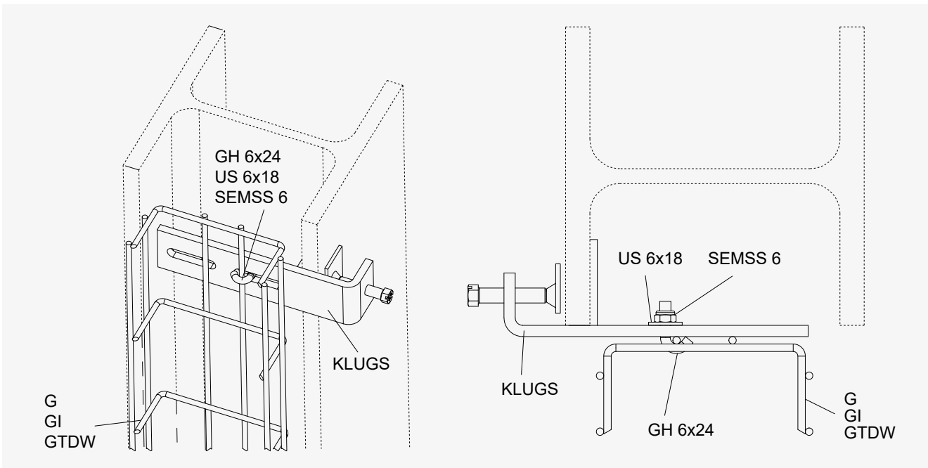
A vertically aligned U-shaped mesh cable tray mounted on a steel beam using the KLUGS fastening clamp set and a bolt set comprising the GH fastening hook, a washer standardised to DIN 125 and a self-locking hexagon nut standardised to DIN 985.
