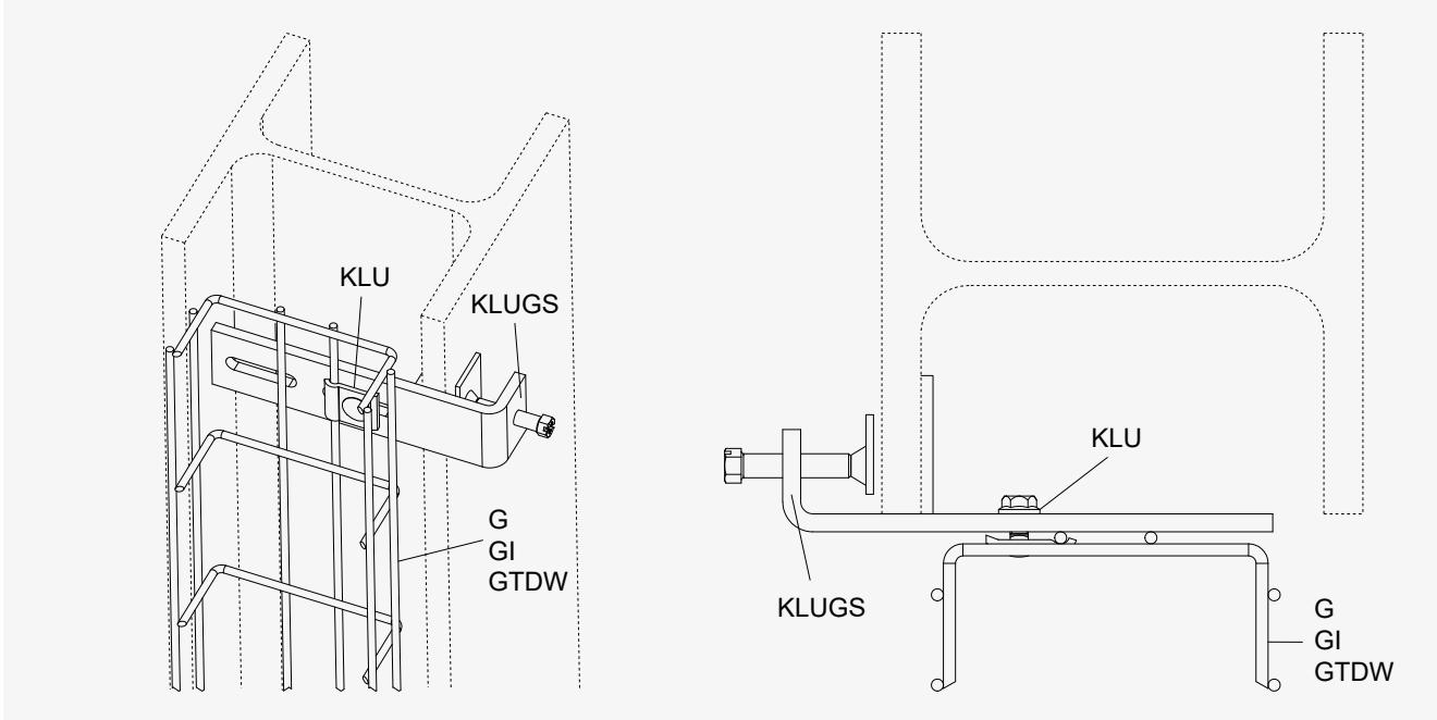
A vertically aligned U-shaped mesh cable tray mounted on a steel beam using the KLUGS fastening clamp set and the KLU clamp fastening set.
