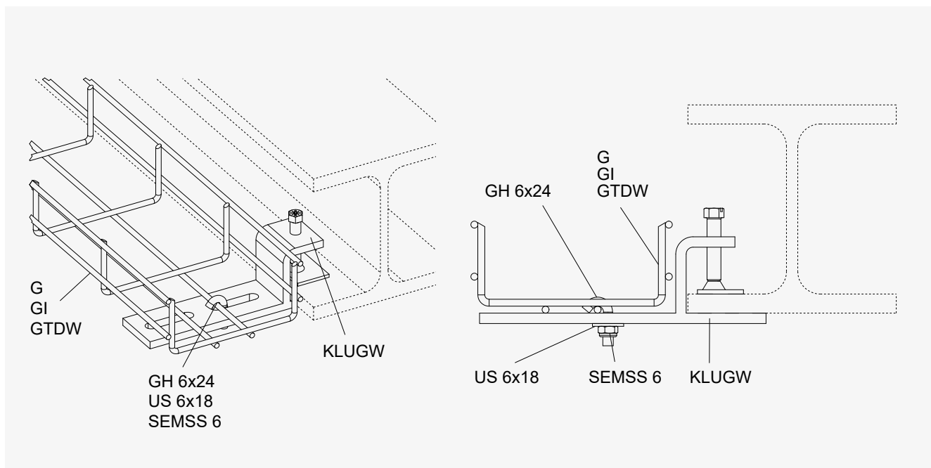
A horizontally aligned U-shaped mesh cable tray mounted on a steel beam using the KLUGW fastening clamp set and a bolt set comprising the GH fastening hook, a standard US DIN 125 washer and a standard SEMSS DIN 985 self-locking hexagon nut.
