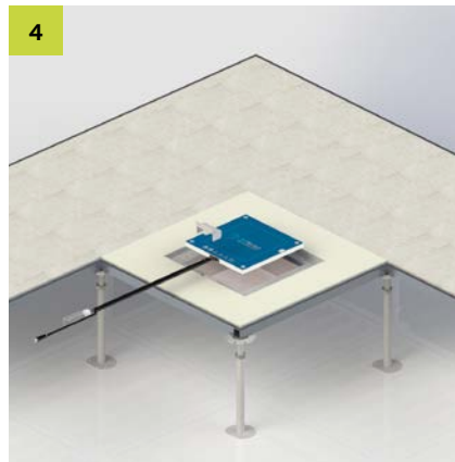
4 Inserting the etaLink3000 charging pad.* The cable must be carefully fed through the opening provided for this purpose in the charging enclosure and to the wallbox*.
