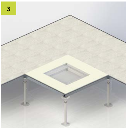
3 If necessary, bolt the WCPS raised floor to the supporting structure.
