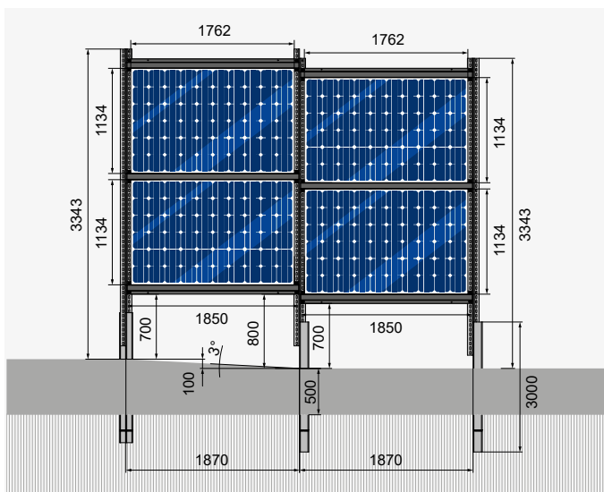
View of solar fence AGRI-PV
